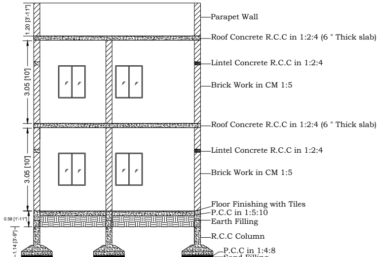
SECTION X-X
