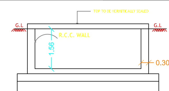
RWH CAPACITY L=5000LTRS
