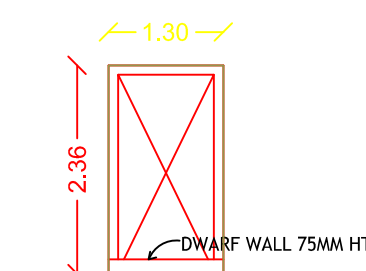
WIKET GATE ELEVATION
