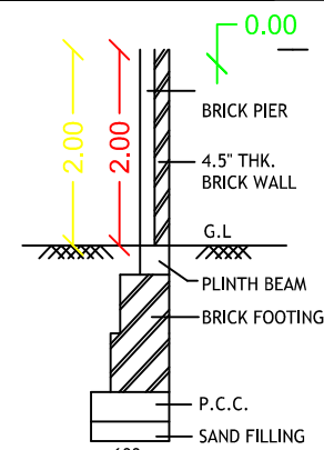
600 COMPOUND WALL DETAIL
