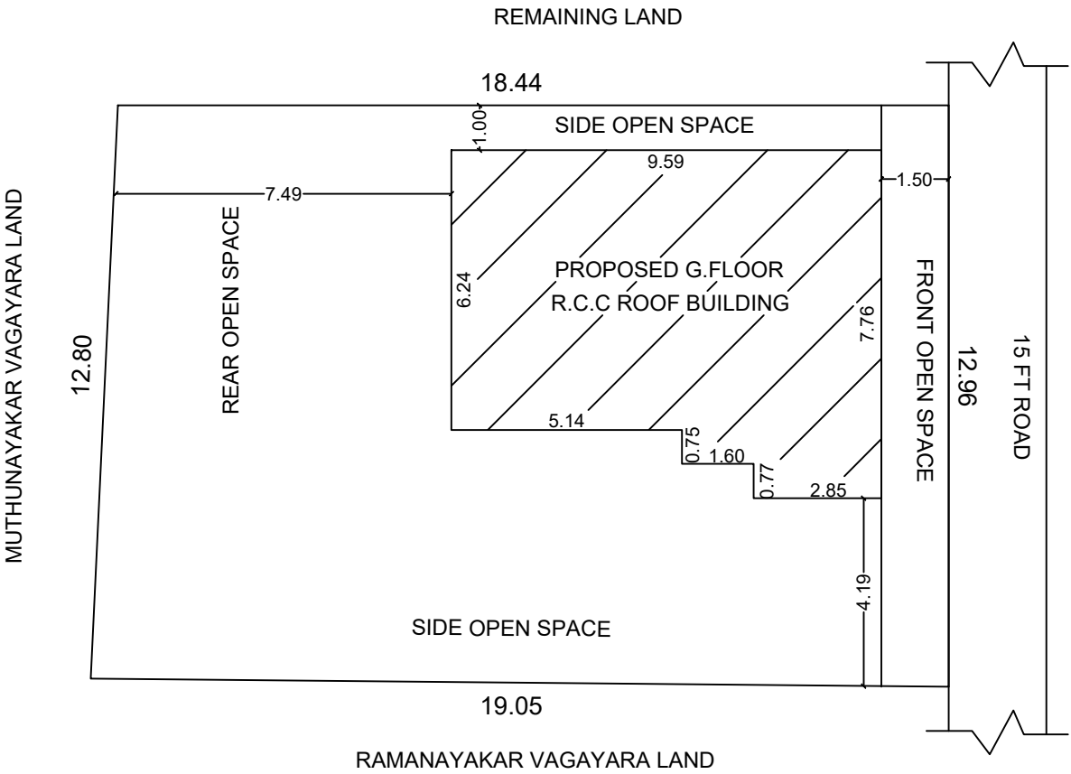
SITE PLAN
