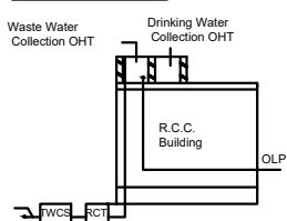
Flow Diagram of Waste Water Recycling & Reuse
