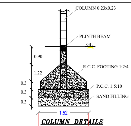
COLUMN DETAILS
