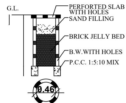
RAIN WATER HARVEST
