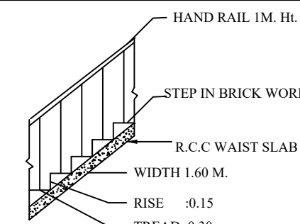
STAIR DETAIL
