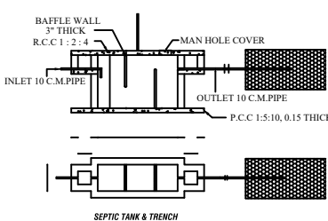
Baffle Wall & Trench
