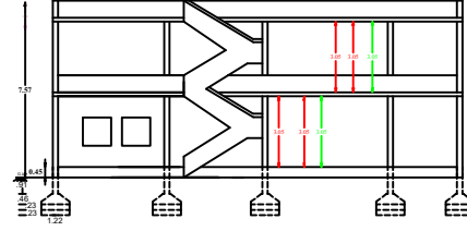
SECTION-AB
