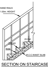
SECTION ON STAIRCASE
