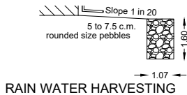
RAIN WATER HARVESTING
