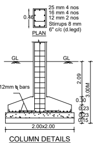
COLUMN DETAILS
