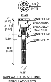
RAIN WATER HARVESTING PERCOLATION PITS
