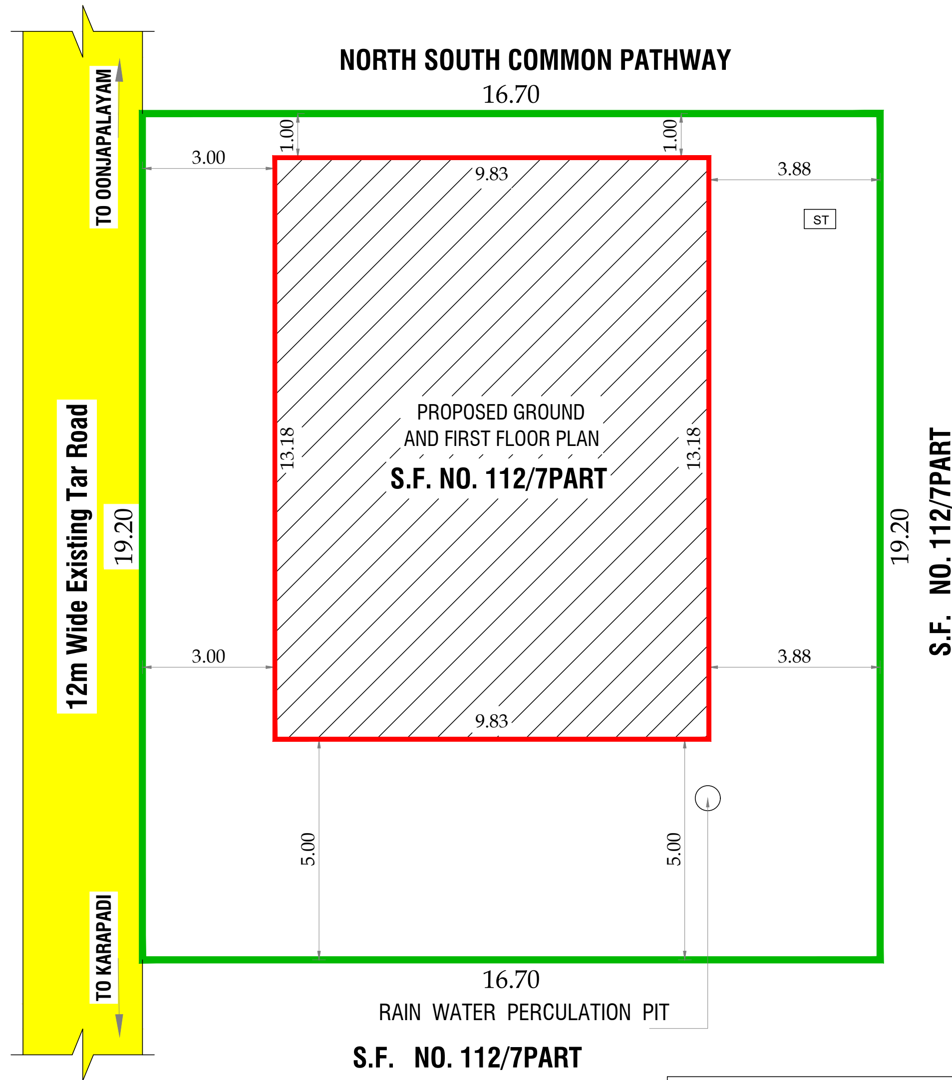
SITE PLAN
