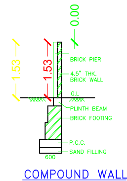
COMPOUND WALL
