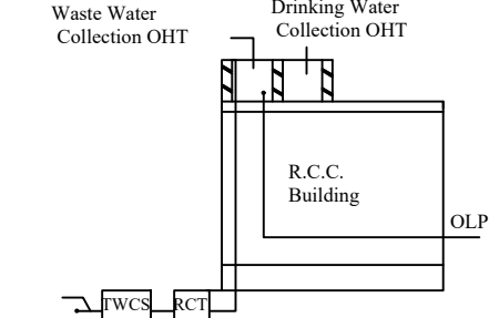
Flow Diagram of Waste Water Recycling & Reuse
