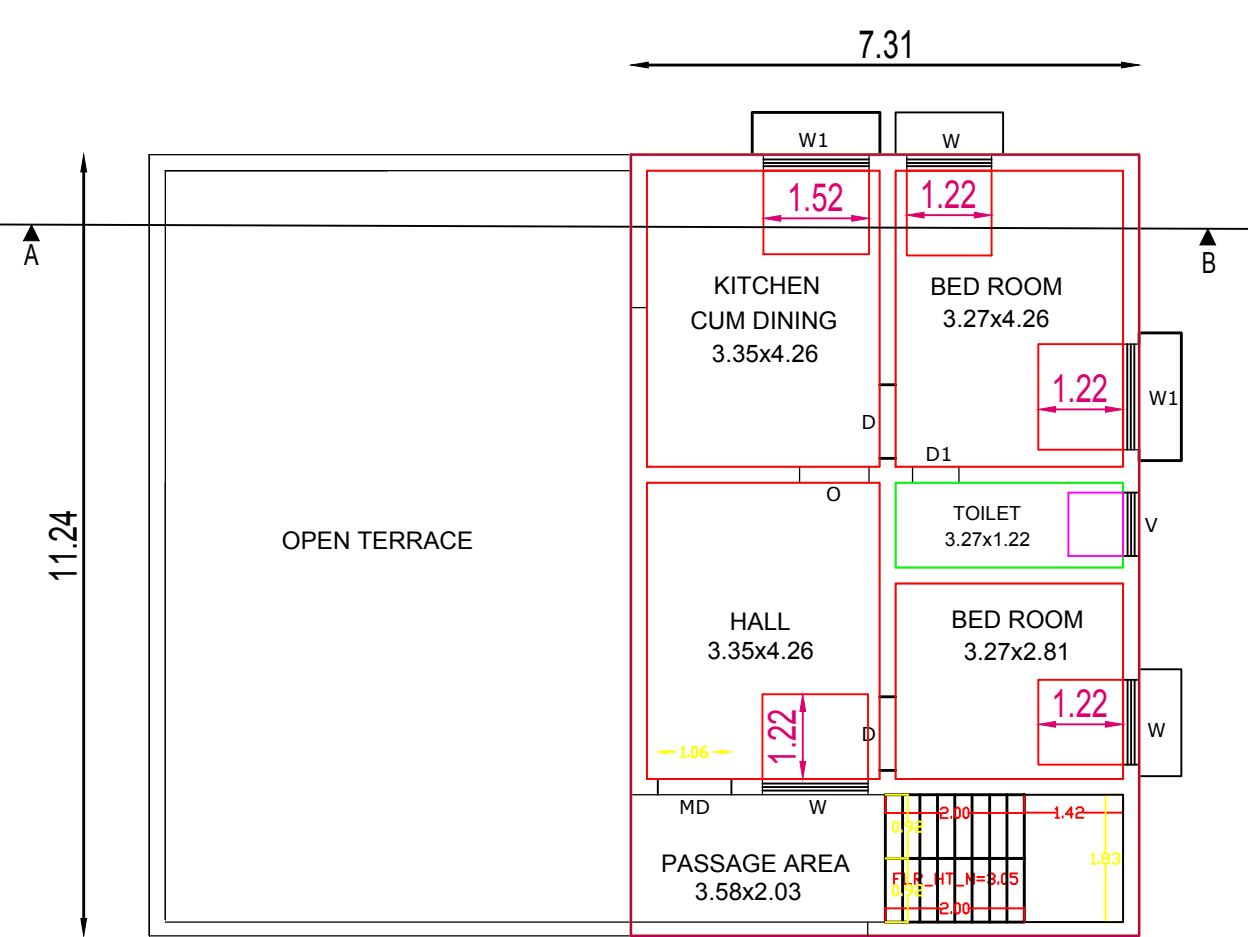
ADDITIONAL PROPOSED SECOND FLOOR PLAN
