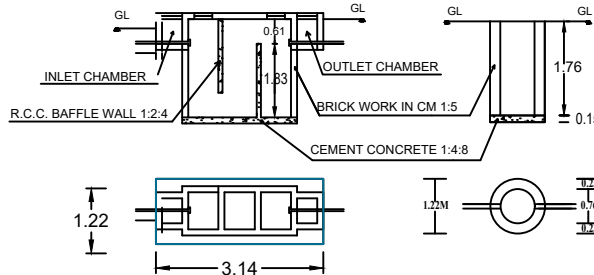
DETAILS OF SEPTIC TANK & SOAK PIT.
