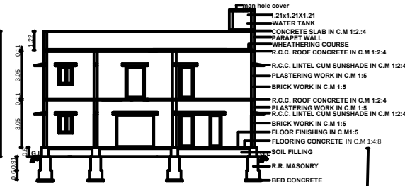
SECTION ON AB & CD
