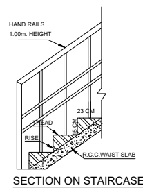
SECTION ON STAIRCASE
