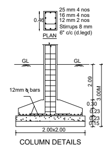
COLUMN DETAILS
