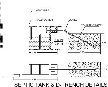
SEPTIC TANK & D-TRENCH DETAILS
