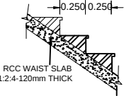
STAIR CASE DETAILS SCALE 1:25
