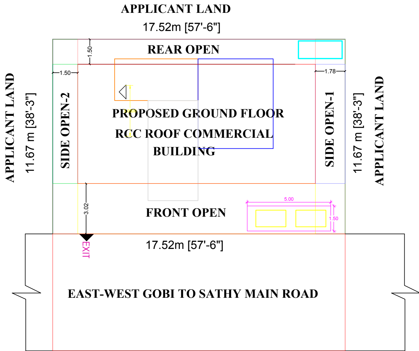
SITE PLAN
