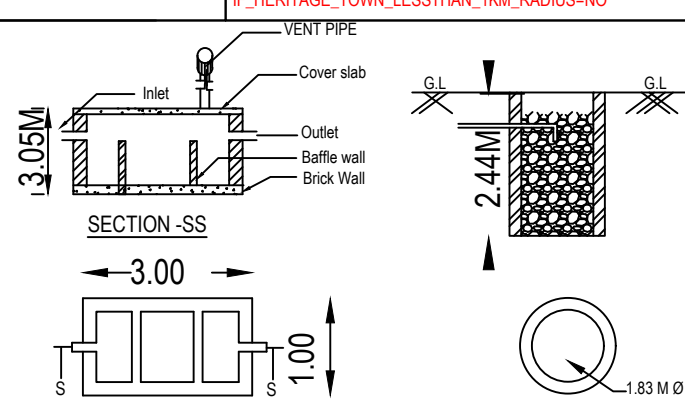
SEPTIC TANK & SOAK PIT DETAILS
