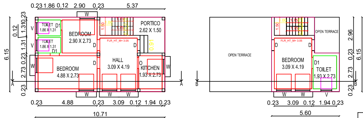
PRO. GROUND FLOOR PLAN
