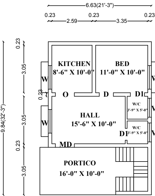
EXL.GROUND FLOOR PLAN
