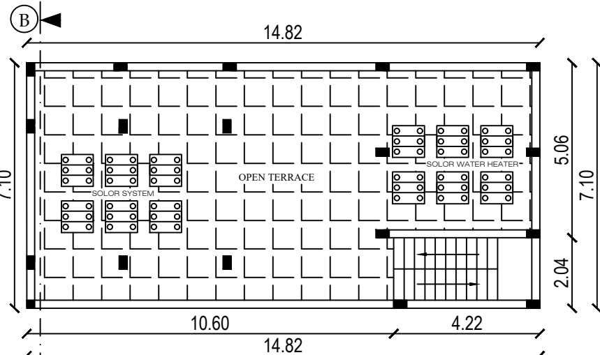
TERRACE FLOOR RCC PLAN
