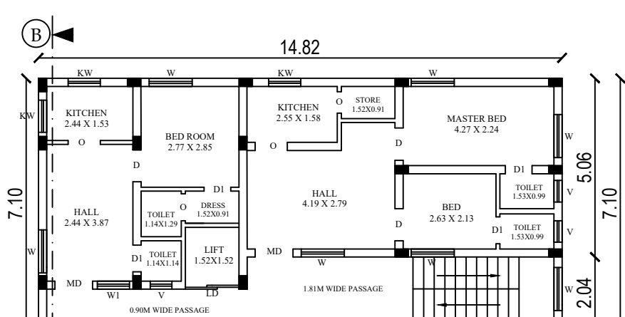
THIRD FLOOR RCC PLAN
