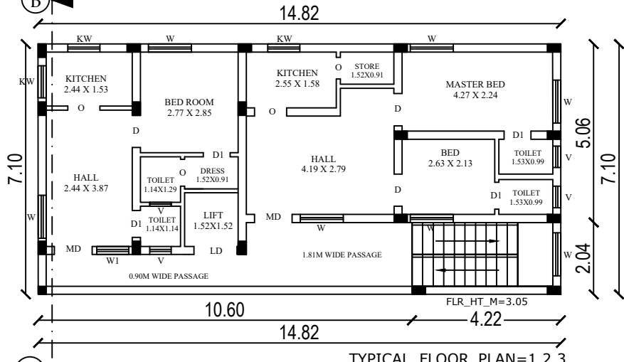
FIRST FLOOR RCC PLAN
