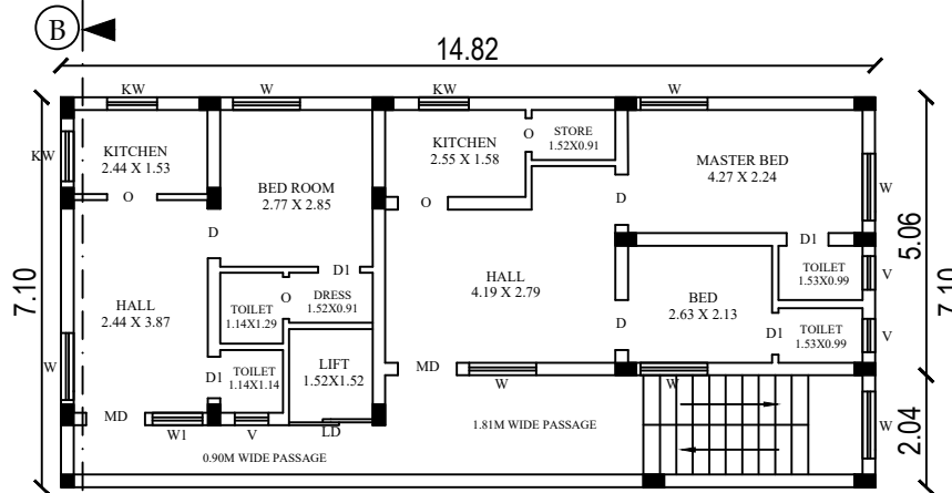
SECOND FLOOR RCC PLAN
