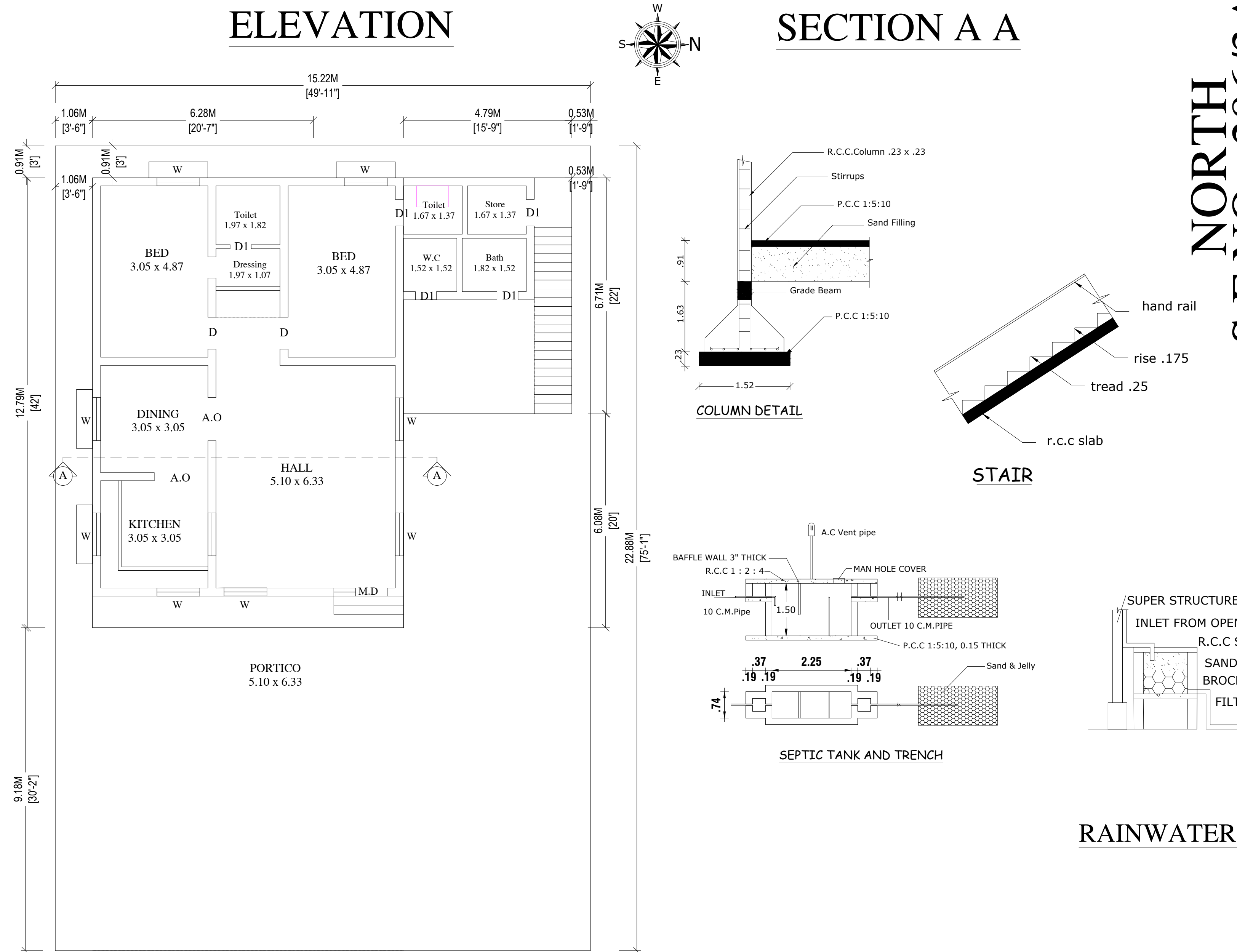
PRO. GROUND FLOOR PLAN
