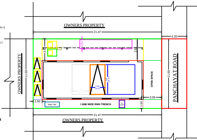
SITE PLAN
