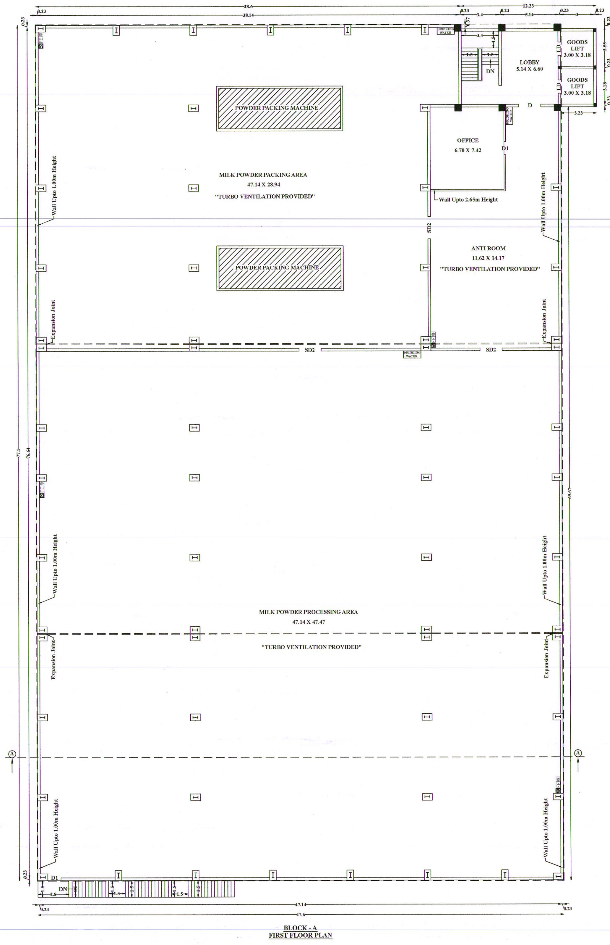
BLOCK - A FIRST FLOOR PLAN
