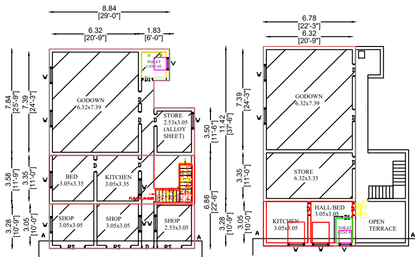
FIRST FLOOR PLAN (PROPOSED-SOUTH)
