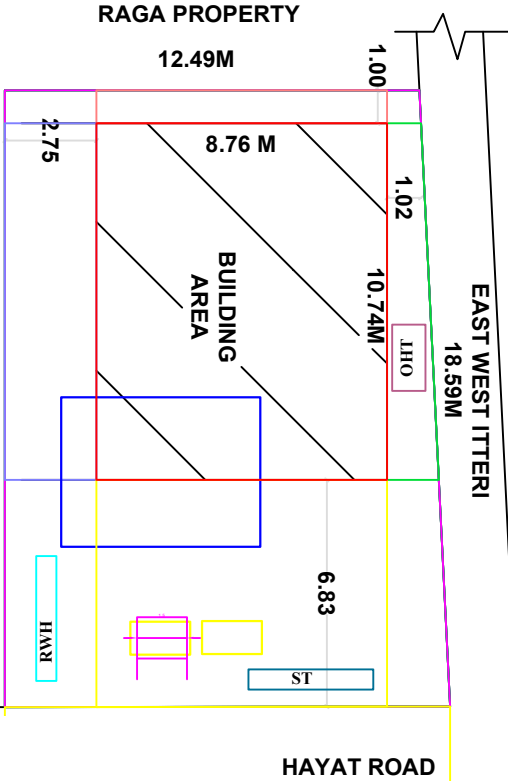
LBP QUARTERS SITE PLAN
