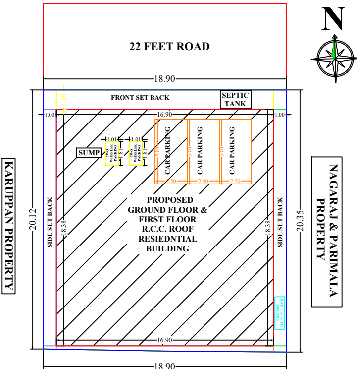
SITE PLAN
