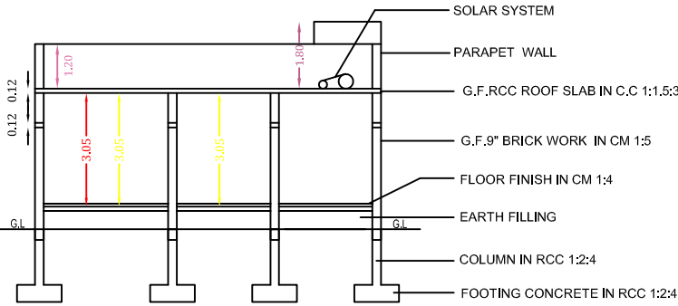
SECTION "AB"
