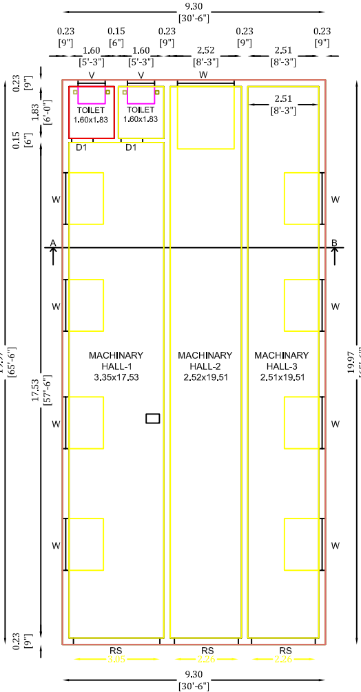
PLAN (SCALE-1:100)
