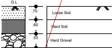
TRIAL PIT DETAILS (NOT TO SCALE)
