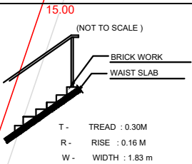
STAIR DETAILS :-
