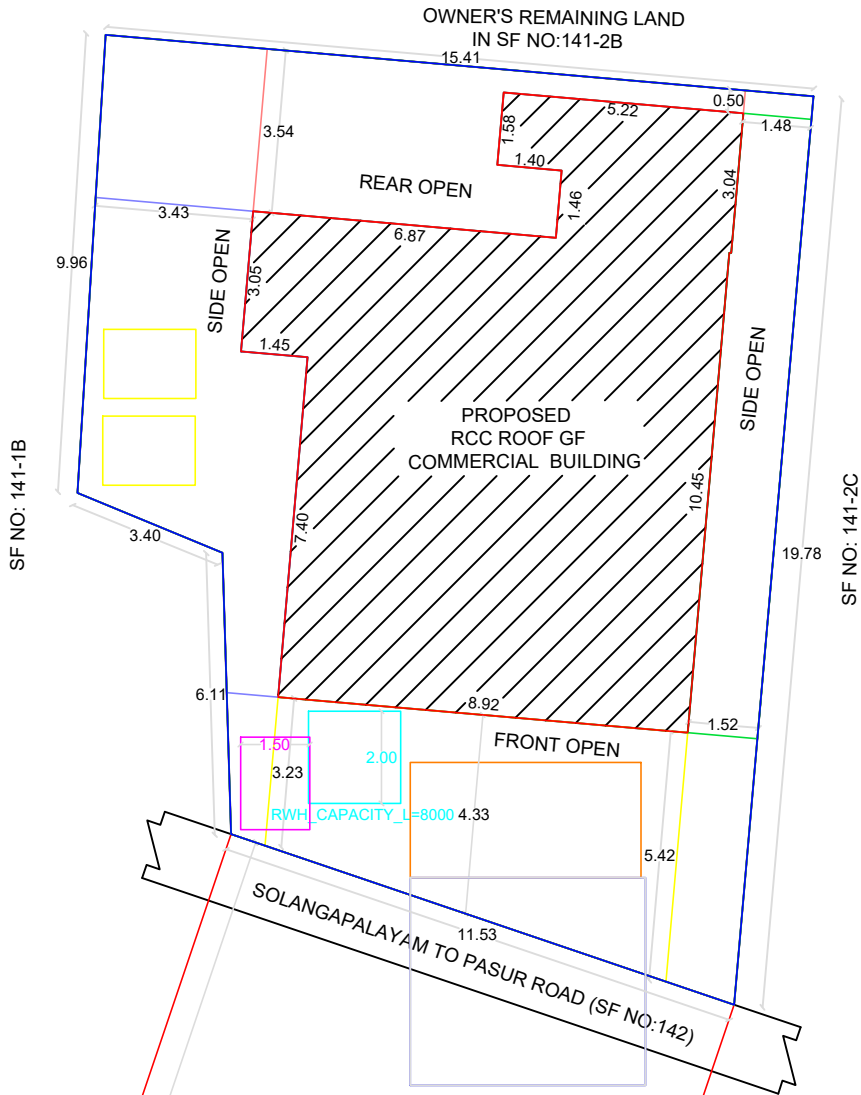
SITE PLAN
