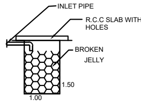
RAIN WATER HARVESTING FILTER BED
