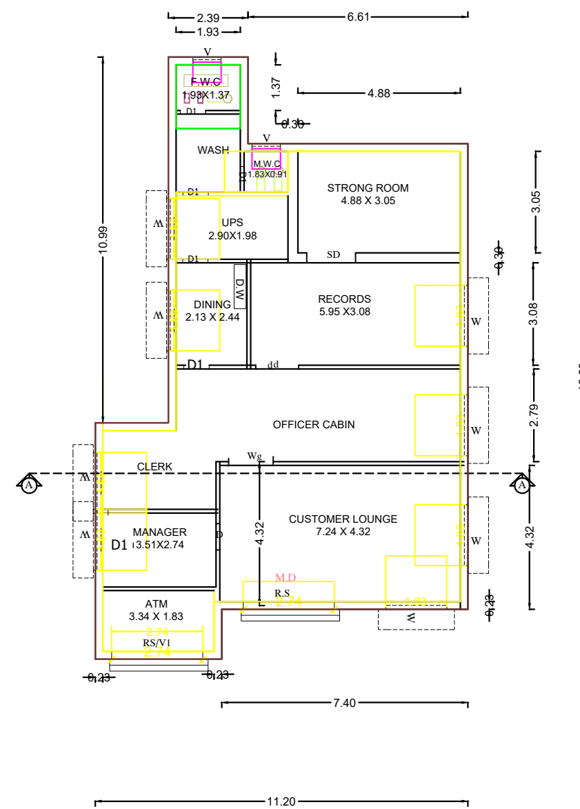
PLAN
