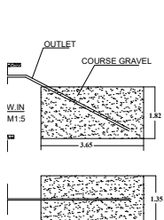
SEPTIC TANK & D-TRENCH DETAILS
