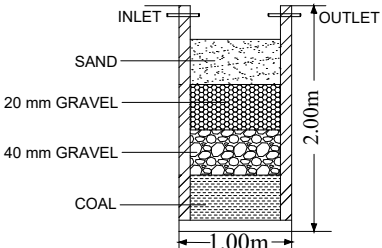
RAIN WATER COLLECTION TANK
