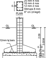
COLUMN DETAILS
