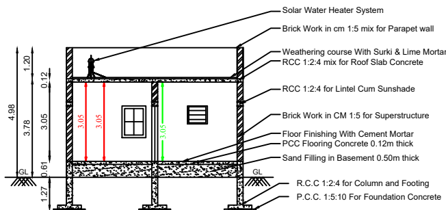
SECTION "AB"
