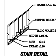
STAIR DETAIL
