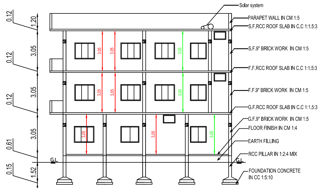
SECTION-"AA"BB"CC"
