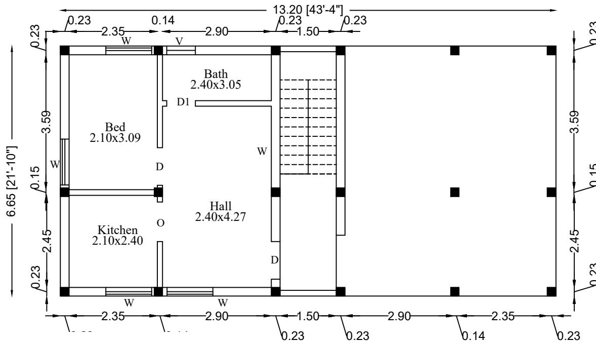
JND FLOOR PLAN
