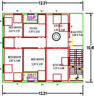
ADD.PRO .FIRST FLOOR PLAN
