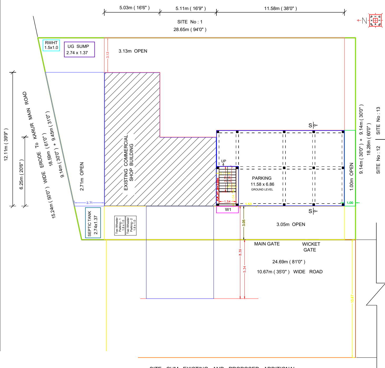
SITE CUM EXISTING AND PROPOSED ADDITIONAL GROUND FLOOR PLAN
