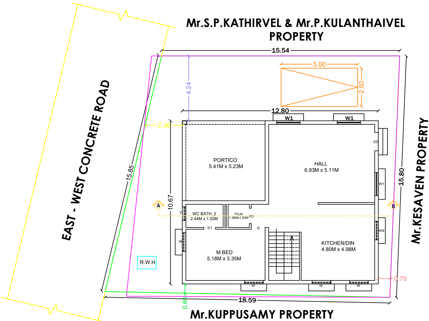
SITE CUM GROUND FLOOR PLAN
