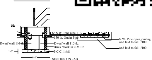
SEPTIC TANK WT.
