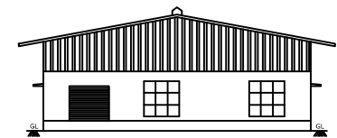
ELEVATION FACING EAST
