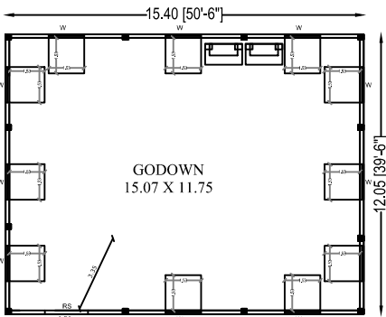
GROUND FLOOR GI SHEET PLAN
