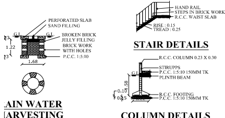
COLUMN DETAILS
