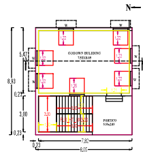
GROUND FLOOR GODOWN BUILDING
