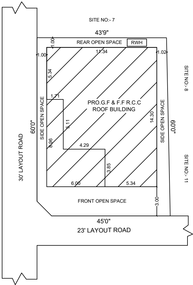
SITE PLAN
