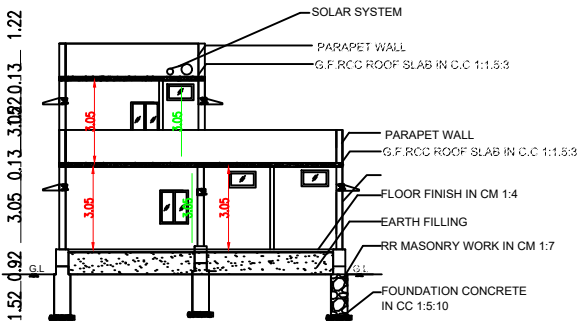
SECTION ON AA & BB
