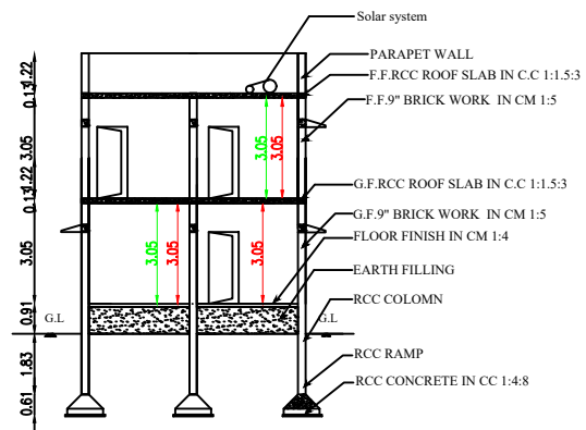
SECTION ON AA& BB
