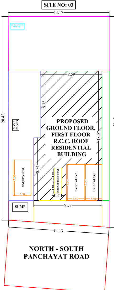
SITE PLAN
