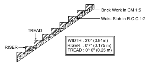
STAIRCASE DETAILS
