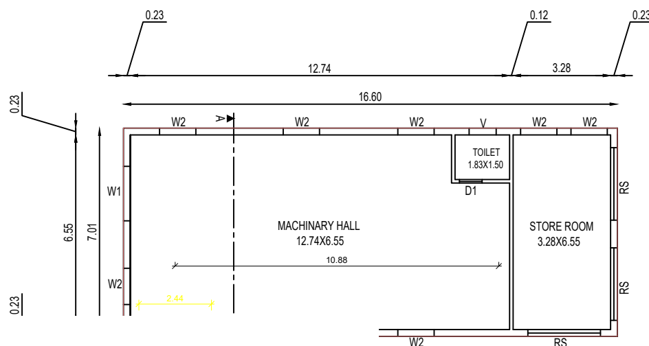
FLOOR PLAN 1:100
