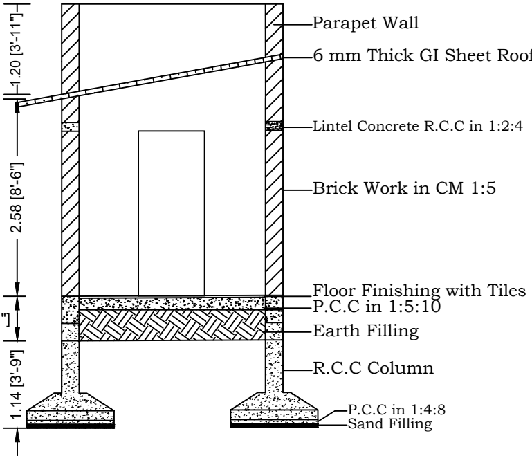
SECTION X-X
