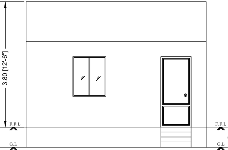
FRONT ELEVATION
