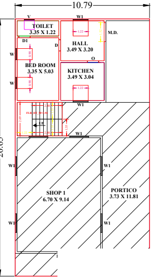
EXISTIN GROUND FLOOR PLAN
