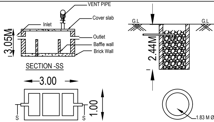
SEPTIC TANK & SOAK PIT DETAILS
