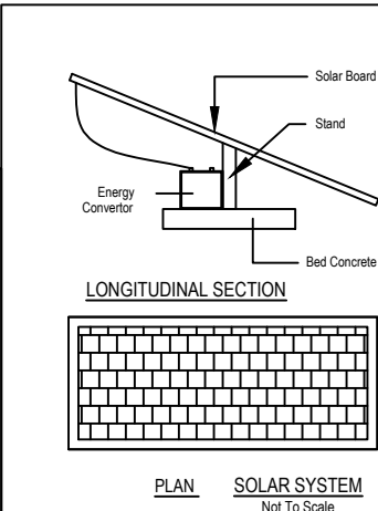
PLAN SOLAR SYSTEM Not To Scale
