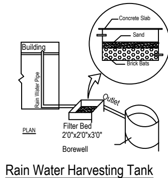
Rain Water Harvesting Tank
