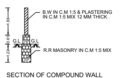
SECTION OF COMPOUND WALL
